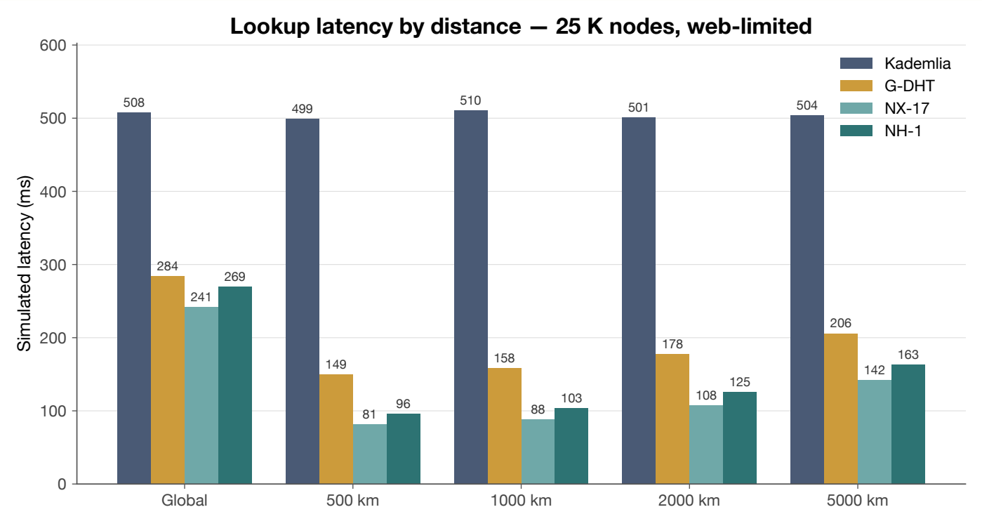
Lookup latency (ms) per distance band, 25 K nodes web-limited. NX-17 (light teal) and NH-1 (deep teal) cluster well below Kademlia (slate) and G-DHT (amber) at every distance.
